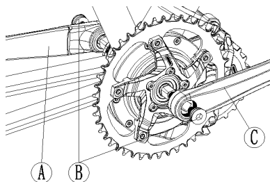
A Left crank B M8 Internal hex screw C Right crank
