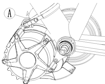
A Hose clamp
