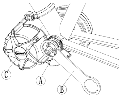
A Locking ring M33-PH1(B) B Special tool
